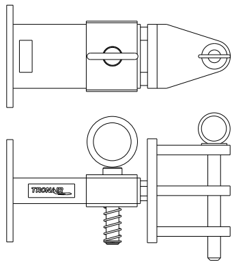
FIGURE 3 01-1950-5000 Standard Telecoupler
